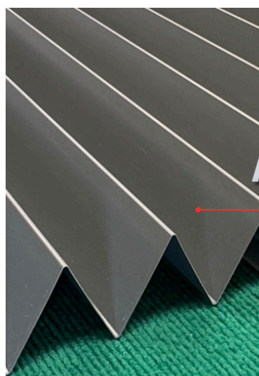
PANEL TYPE : W350A Rib height 59 mm. wide 350 mm.
